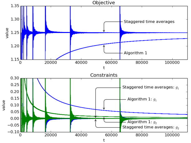
Fig. 2. Processes of solving (49) with f(x) = 1.5x_1 + x_2
