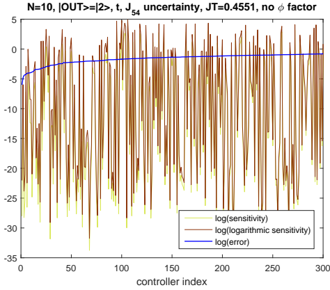
Fig. 4: Case N = 10 , |\text{OUT}\rangle = |2\rangle , J_{54} uncertain, with S(t) defined by (11)
