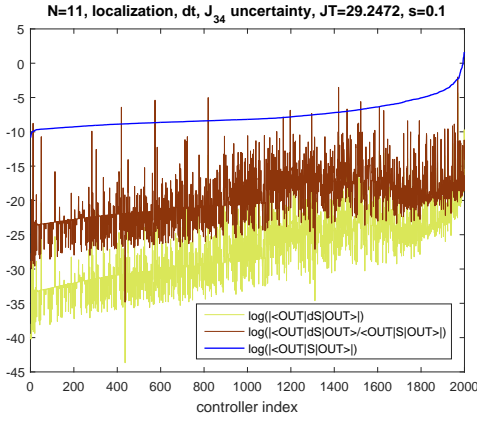
Fig. 7: Case N = 11 , |\text{OUT}\rangle = |1\rangle , J_{34} uncertainty, \hat{S}(s) defined as in Eq. (13), with phase factor
