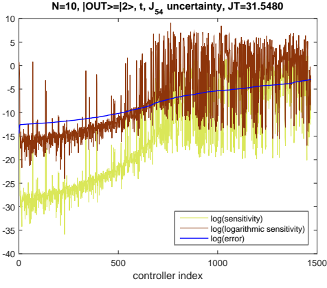
Fig. 3: Case N = 10 , |\text{OUT}\rangle = |2\rangle , J_{54} uncertain, with S(t) defined by (7)
