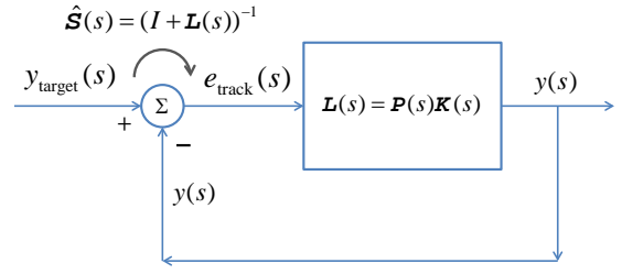
Fig. 1: Classical single-degree-of-freedom loop
