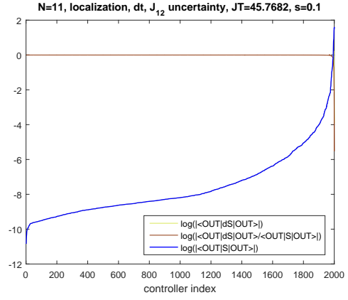
Fig. 5: Case N = 11 , |\text{OUT}\rangle = |1\rangle , J_{12} uncertainty, \hat{S}(s) defined as in Eq. (13), with phase factor
