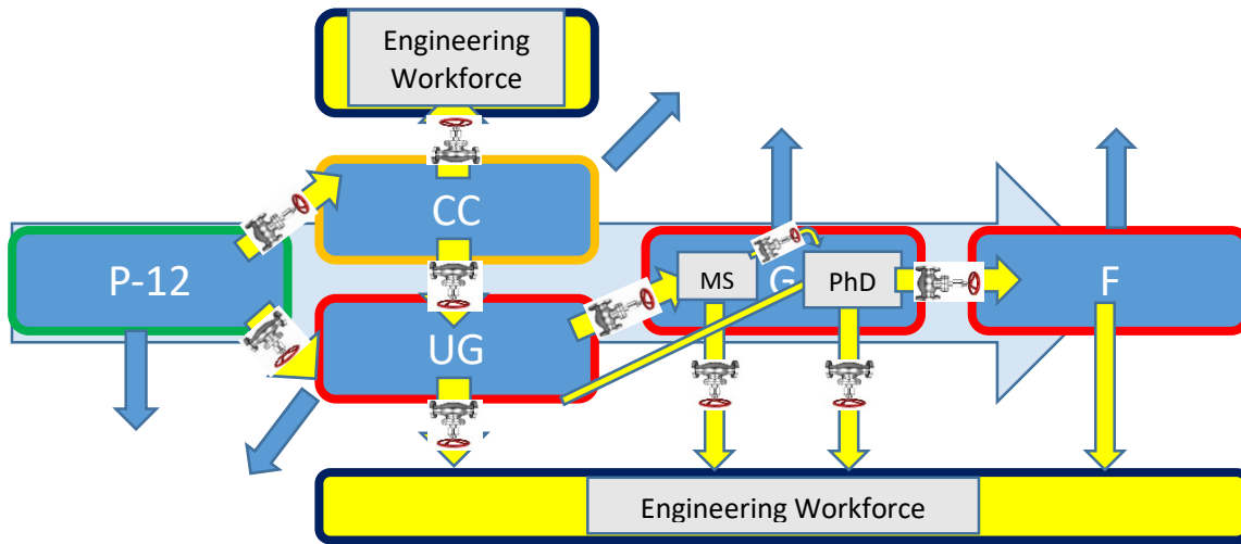
Figure 1: A schematic description of the engineering “pipeline” in terms of a flow process consisting of interconnected control volumes.
